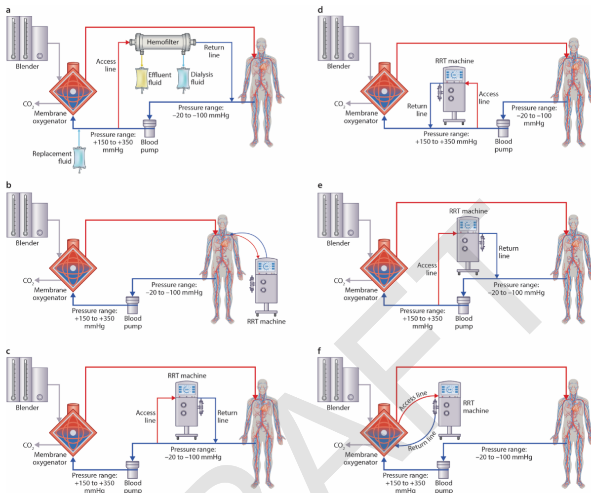
Figure 19 | Options of combining ECMO and CRRT circuits. 1068 a. An in-line hemofilter is integrated into the ECMO circuit. Replacement fluid is directly administered into the ECMO circuit. Alternatively, dialysis fluid can be supplied in a counter-current position. Replacement/dialysis fluid rates and ultrafiltration rates can be controlled via infusion pumps. b. The CRRT device is connected to the patient through a separate catheter independent of the ECMO circuit. c. The access (inlet) and the return (outlet) lines of the CRRT device are connected before the centrifugal blood pump (low-pressure part) of the ECMO circuit. d. Both the access and the return lines of the CRRT device are connected after the blood pump. e. The access line of the CRRT device is connected after the blood pump (high-pressure), while the CRRT return line is connected before the centrifugal blood pump. f. The access line of the CRRT device is connected directly after the membrane oxygenator, while the return line is connected directly before the oxygenator. CRRT, continuous renal replacement therapy; ECMO, extracorporeal membrane oxygenation.
