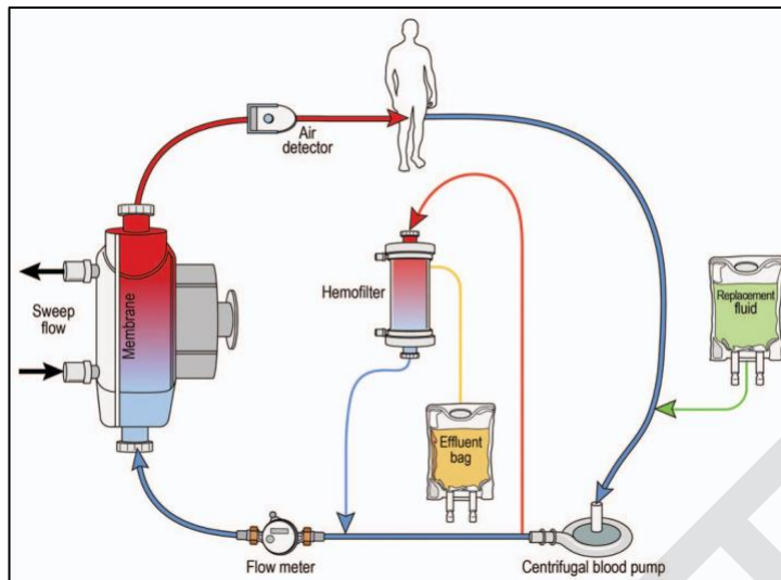
Figure 18 | Configuration of in-line hemofilter integration into ECLS circuit. 1062 ECLS, extracorporeal life support
